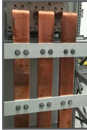
ANA BARA SABİTLEME FIXING TO MAIN BUSBAR
